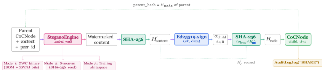
Figure 5: Document sharing cryptographic data flow
