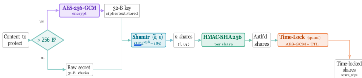
Figure 7: Access control cryptographic data flow
